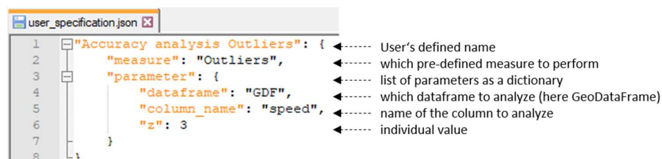
Fig. 3: Example of the JSON specification file as configuration for the tool
